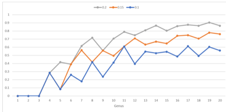
Figure 1: Proportion of S \in \mathcal{S}_g with |e(S) - \frac{1}{5}g| < \epsilon g . Plotted for \epsilon = 0.2 , \epsilon = 0.15 and \epsilon = 0.1 .
